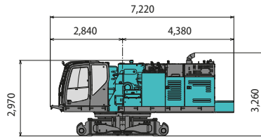
Base machine (without counterweight, without crawler)
